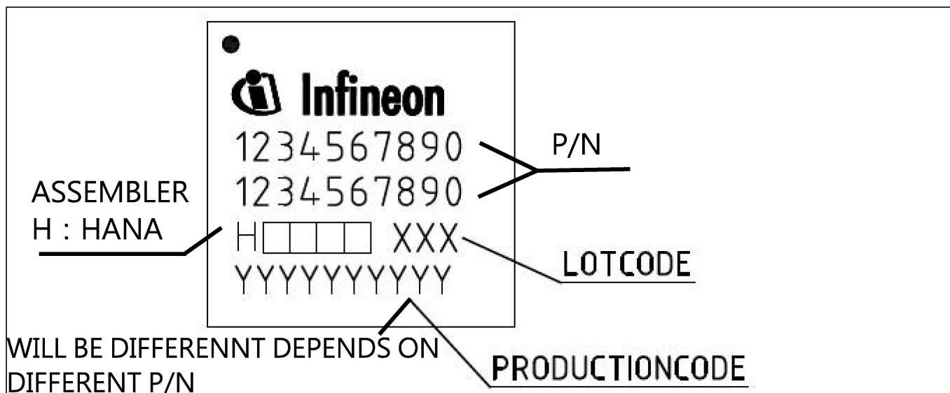
Figure 67 Package Marking
