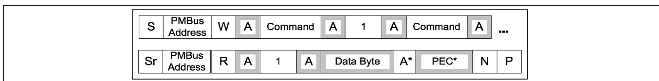
Figure 63 Block Read Process Call
