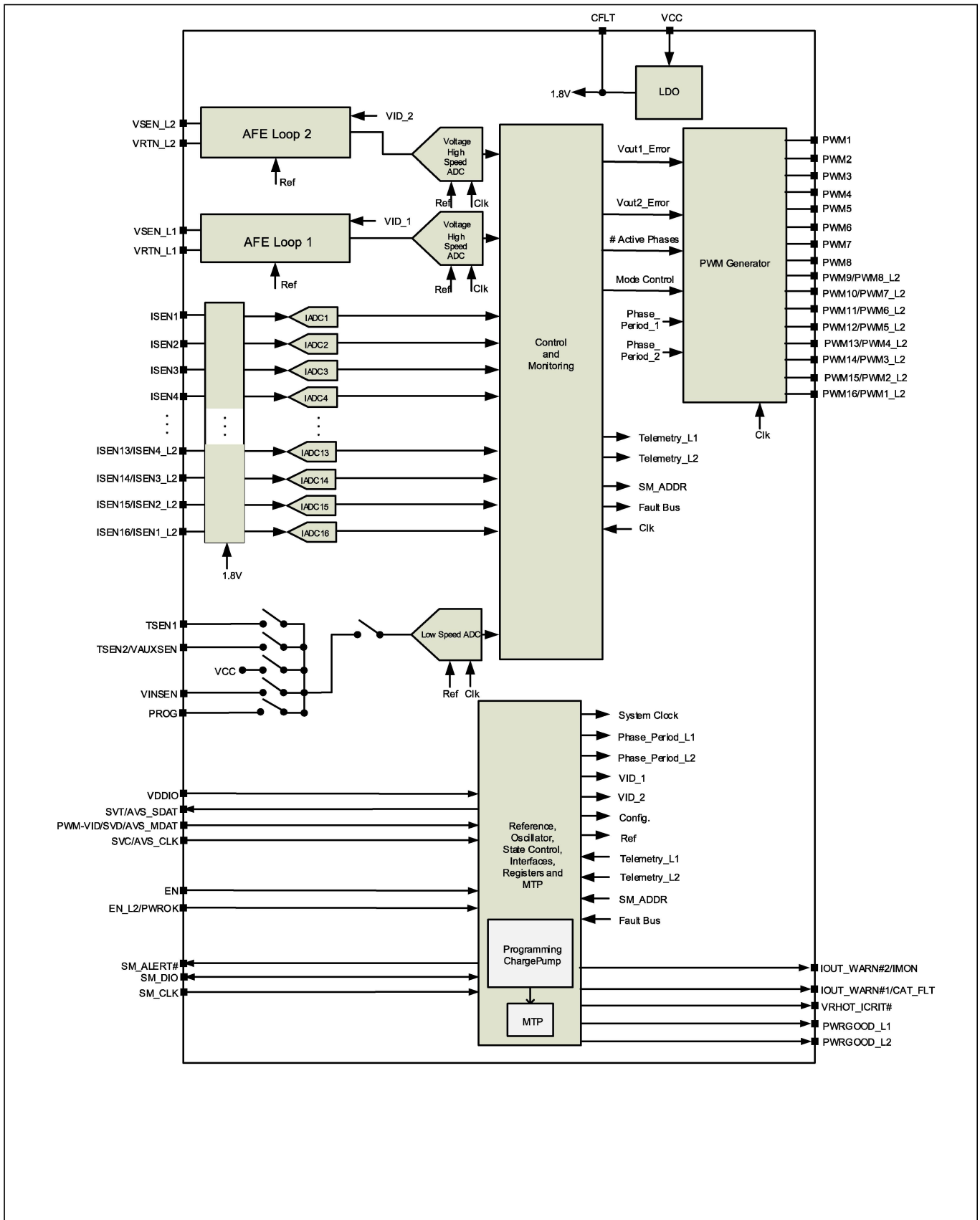
Figure 2 Block Diagram
