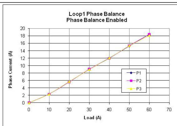
Figure 23 Typical Phase Current Balance (3-Phases enabled)
