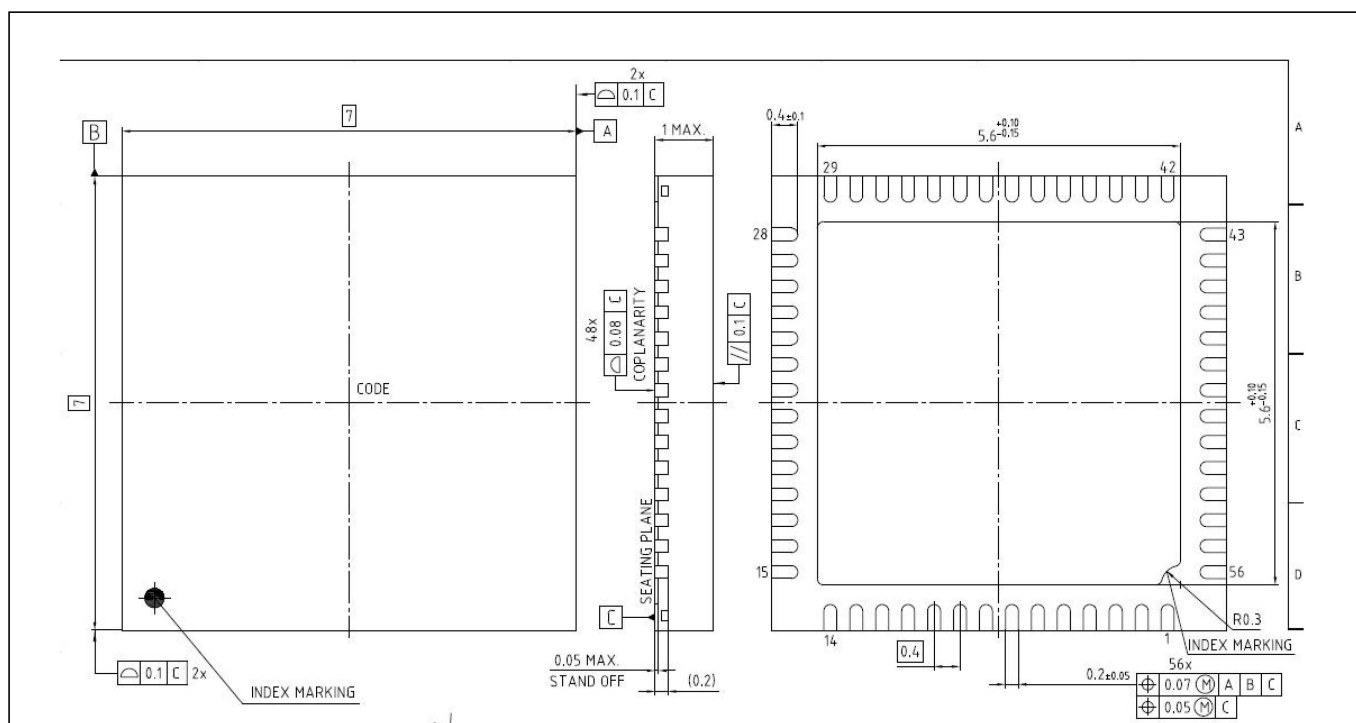
Figure 68 Package Dimensions
