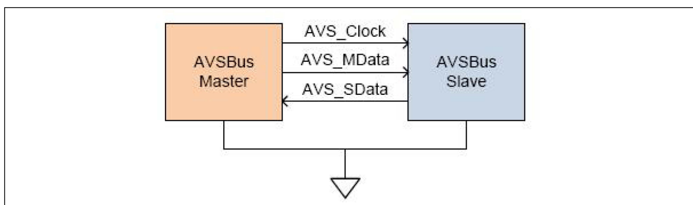
Figure 43 AVSBus 3-wire Interface
