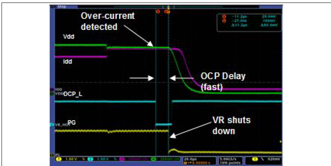
Figure 48 OCP_L (VR_HOT) assertion with OCP_spike (Fast) threshold. OCP delay action (11μs)
