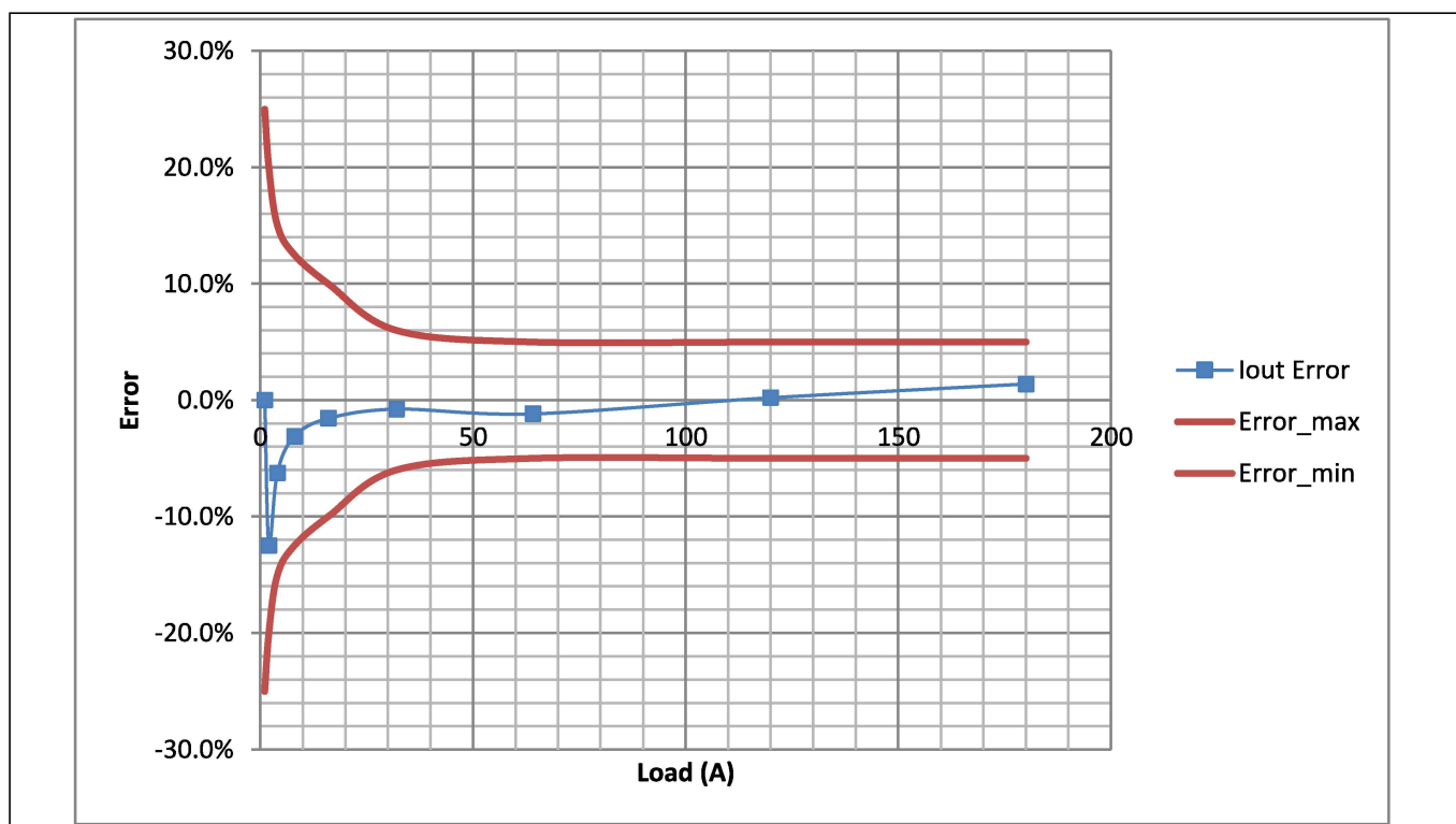
Figure 41 IOU Error using Power Stage Iout
