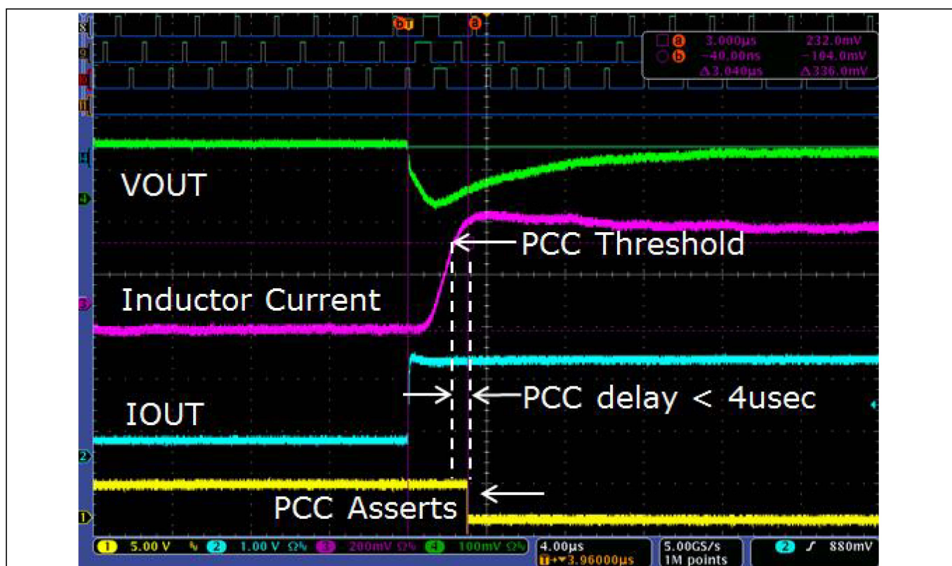
Figure 49 PCC assertion delay due to inductor current lag time
