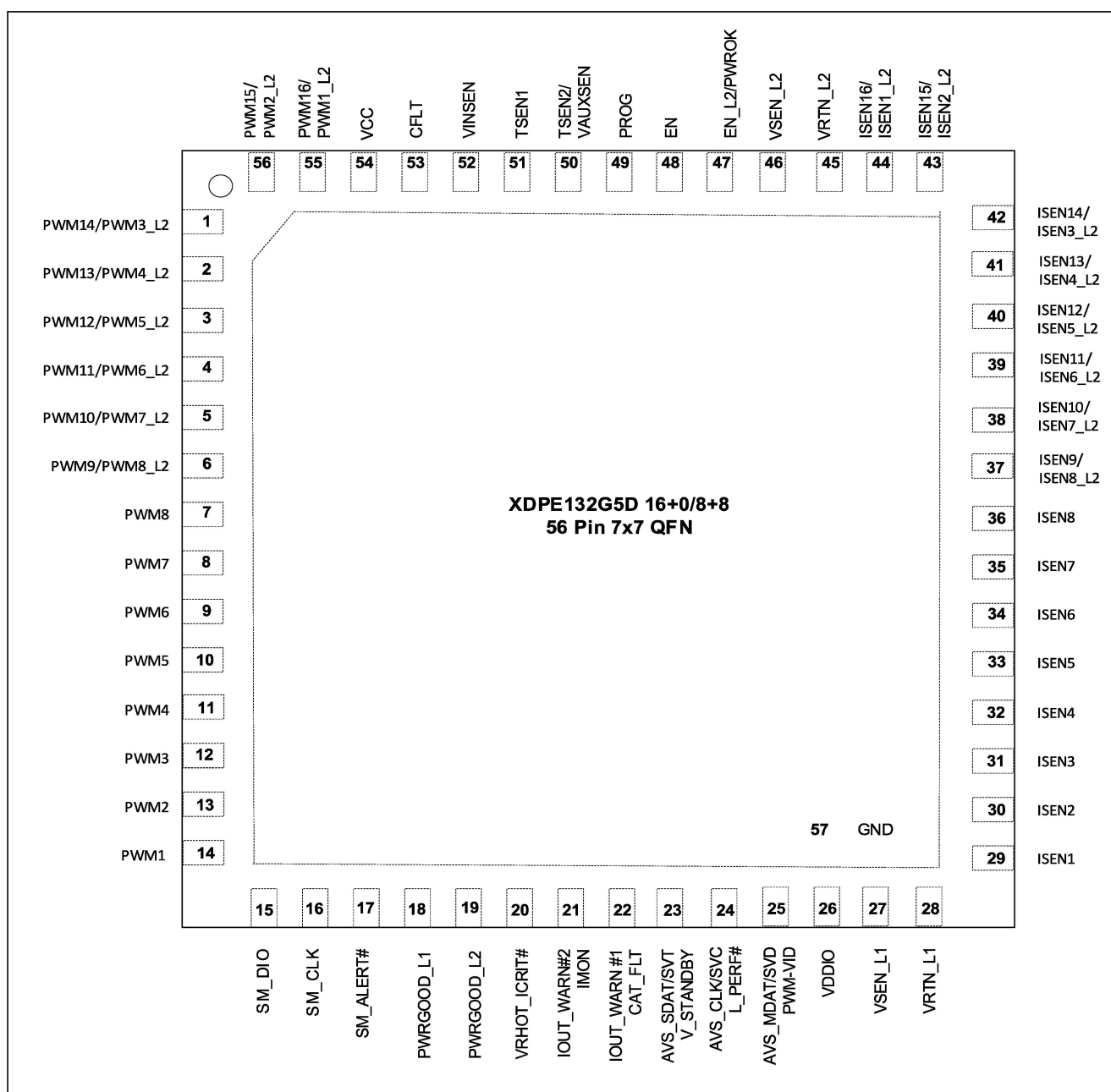
Figure 1 Package Top View
