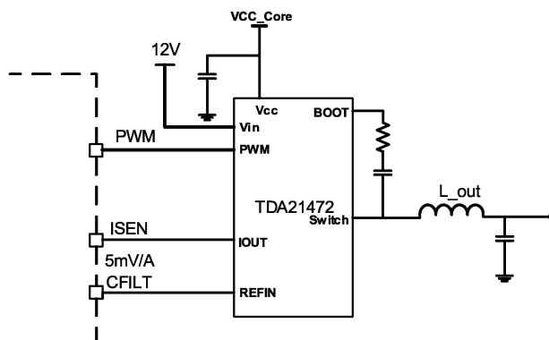
Figure 22 RDson Current Sense
