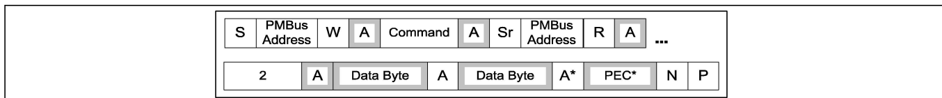
Figure 58 PMBus Block Read with Byte Count = 2
