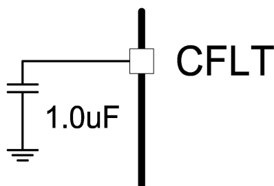
Figure 10 CFLT 1.8 V Decoupling
