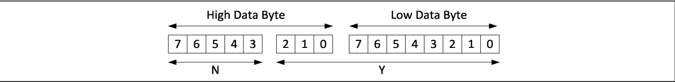
Figure 65 11-bit Linear Data Format
