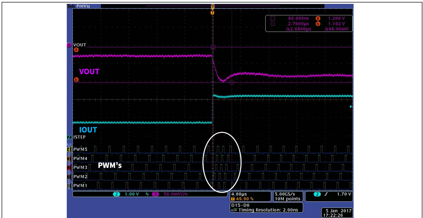
Figure 26 ATA Feature – Zoomed In
