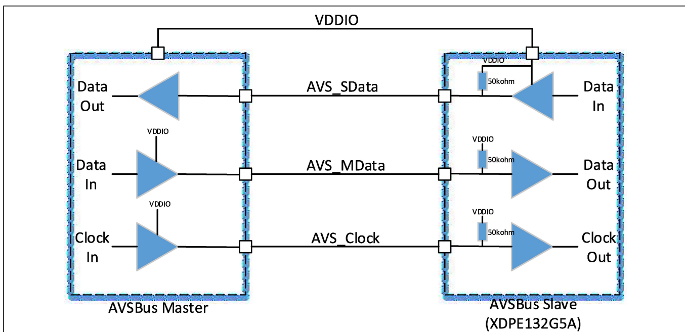
Figure 45 Electrical Interface
