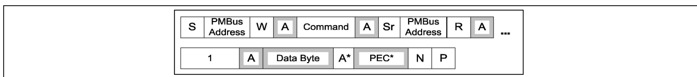
Figure 57 PMBus Block Read with Byte Count = 1
