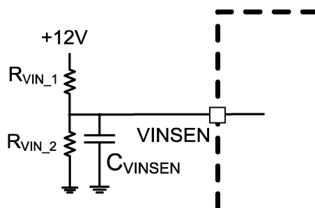
Figure 11 VINSEN Resistor Divider Network
