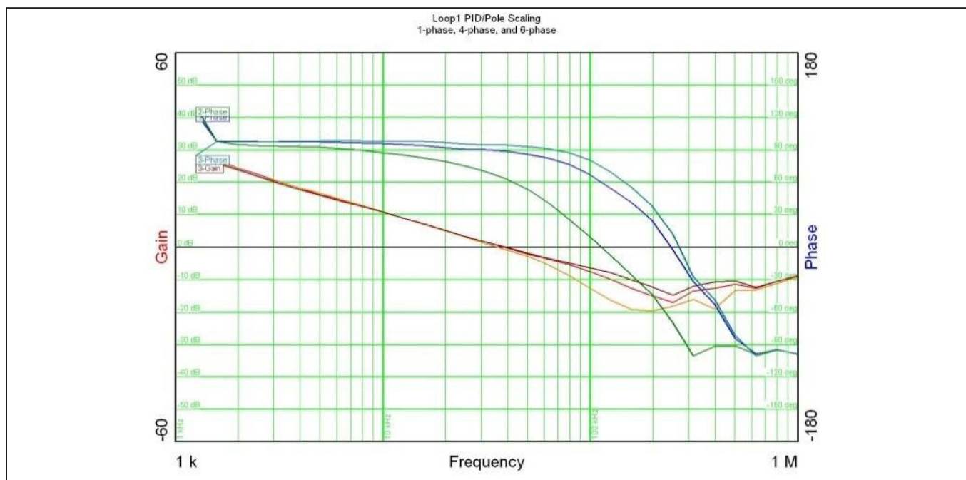
Figure 24 Stability With Phase Add/Drop
