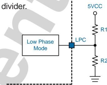
Figure 3. Circuit of LPC Setting
