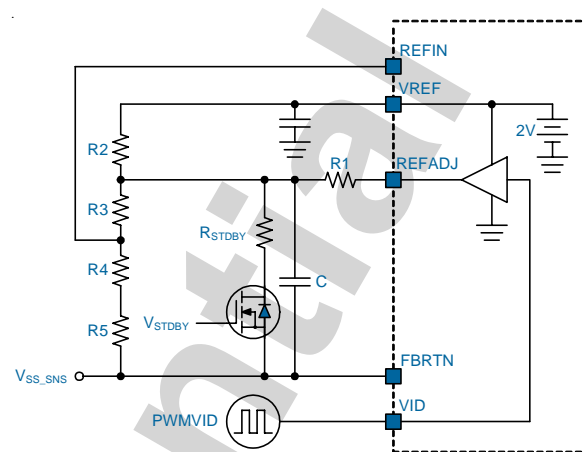
Figure 8. PWMVID structure
