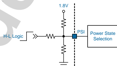
Figure 2. PSI application circuit
