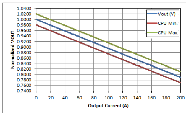
Figure 32: Load Line Measurements
