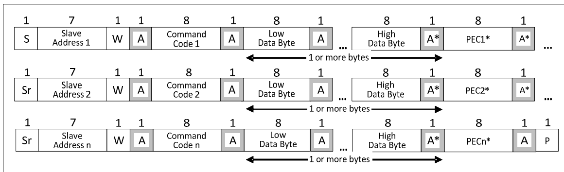
Figure 64: Group Command
