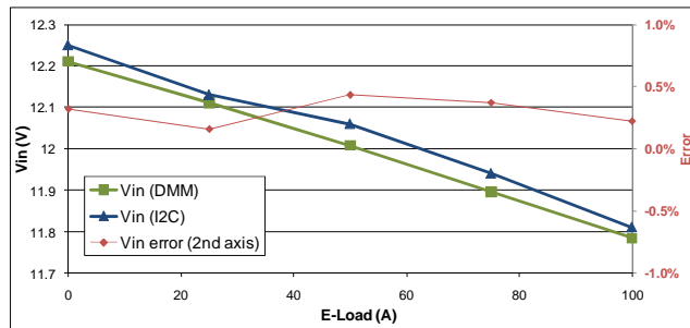
Figure 51: I2C Input Voltage Measurements
