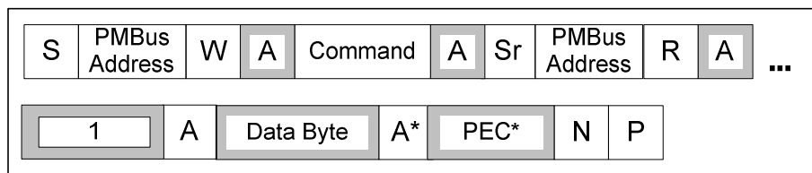
Figure 57: PMBus Block Read with Byte Count=1
