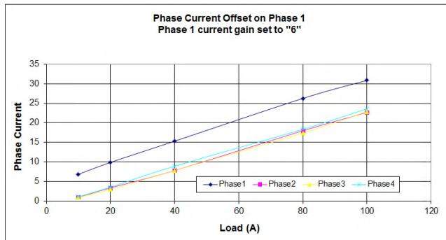
Figure 29: Phase 1 Current Offset
