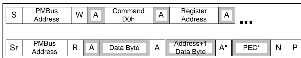
Figure 62: MFR_READ_REG
