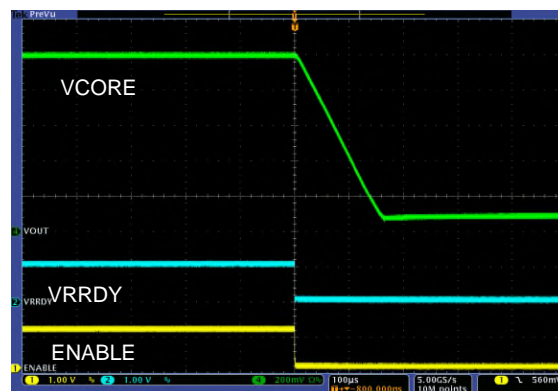
Figure 13: Enable-based Shutdown
