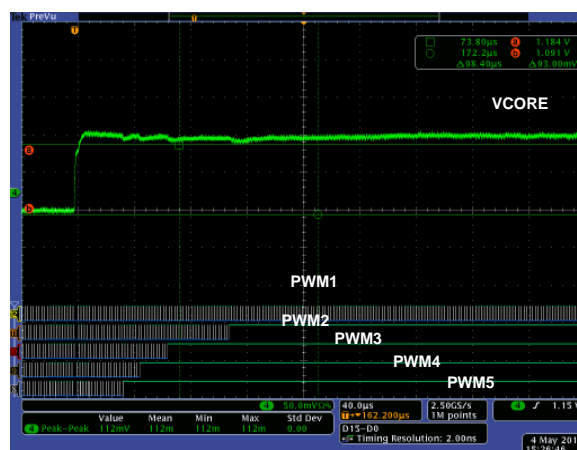
Figure 39: Phase Shed 4Φ→1Φ
