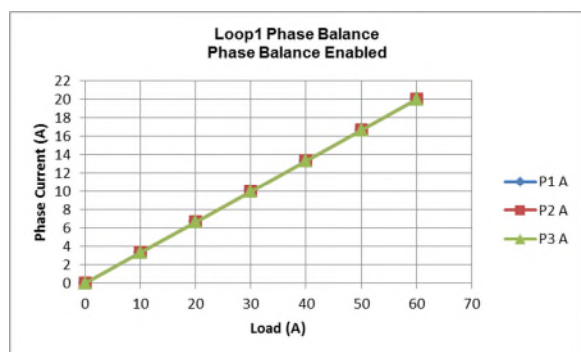
Figure 28: Typical Phase Current Balance (3-phases enabled)
