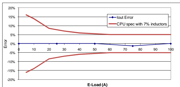
Figure 50: I2C IOUT Error using 10% DCR Inductors
