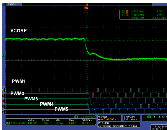
Figure 40: Phase Add 1Φ→4Φ
