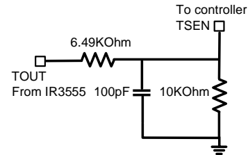
Figure 48: Temperature Sense IR Power Stage Network
