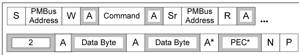
Figure 58: PMBus Block Read with Byte Count=2
