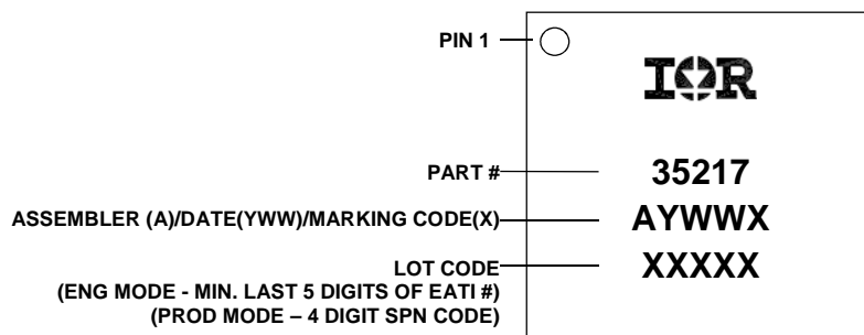
Figure 67: Package Marking
