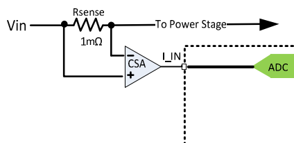
Figure 25: Input Current Sensing
