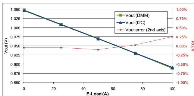
Figure 52: I2C Output Voltage Measurements
