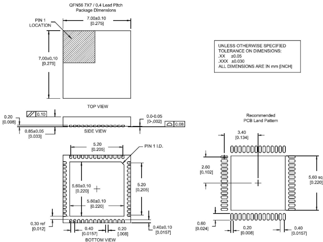
Figure 68: Package Dimensions
