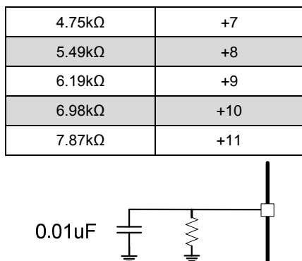
Figure 16: ADDR Pin Components
