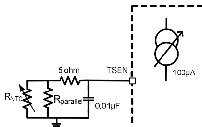
Figure 47: Temperature Sense NTC Network
