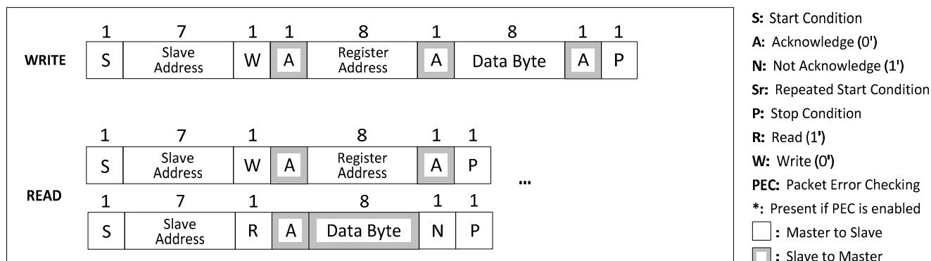
Figure 53: I2C Format
