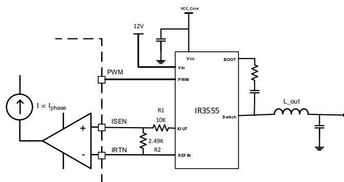
Figure 27: R_{DS(ON)} Current Sense
