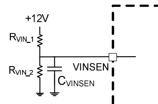
Figure 10: VINSEN resistor divider network
