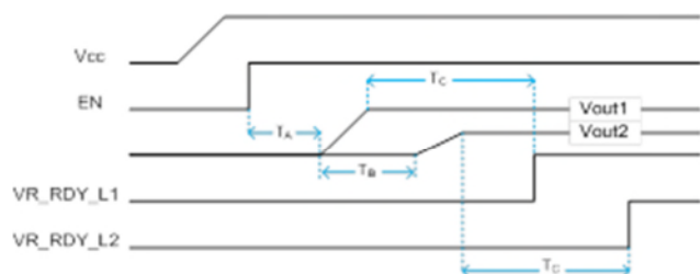
Figure 11: MPoL Startup
