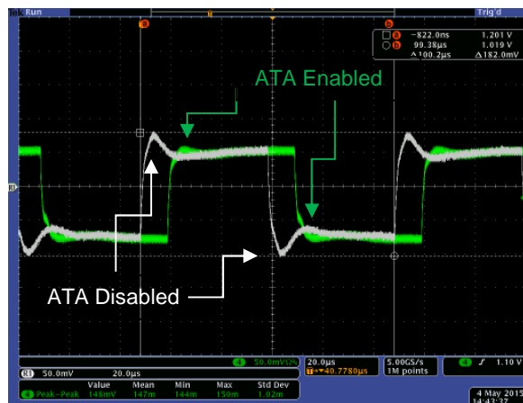
Figure 34: ATA Enable/Disable Comparison
