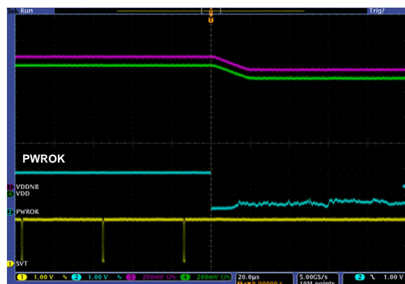
Figure 14: PWROK De-assertion
