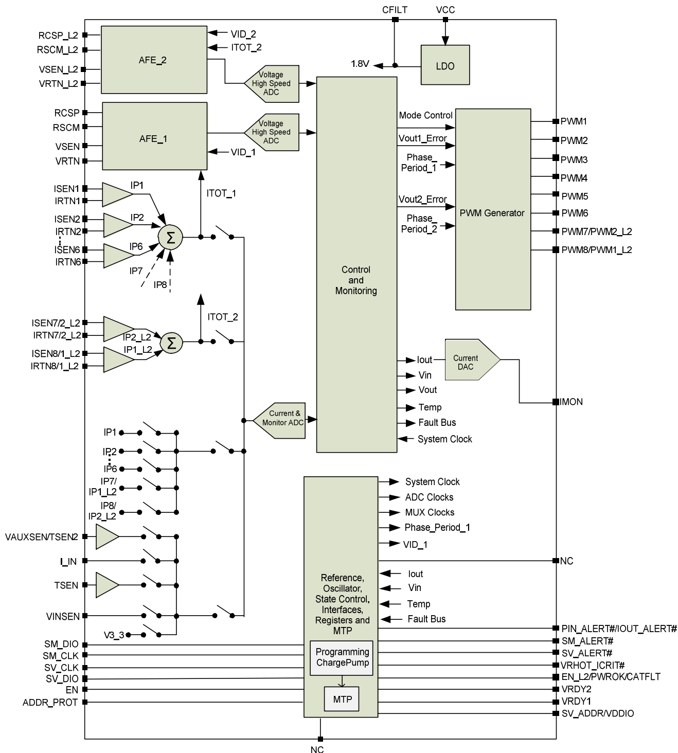
Figure 2: IR35217 Block Diagram
