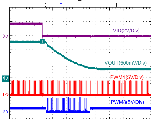
VID = High to Low
