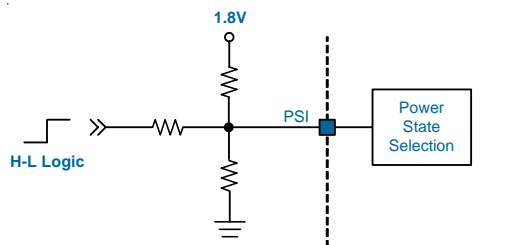
Figure 8. PSI Application Circuit
