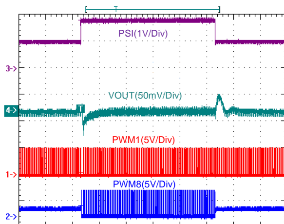
PSI = 1V \pm 1.8V
