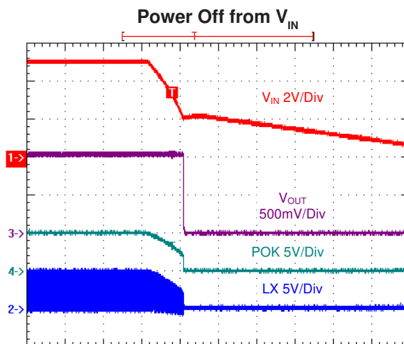
Time (4ms/Div) V_{IN} = 5V , V_{OUT} = 1.05V , I_{OUT} = 3A
