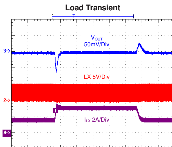
Time (100us/Div) V_{IN} = 5.0V , V_{OUT} = 1.8V , I_{OUT} = 1.5A \sim 3A
