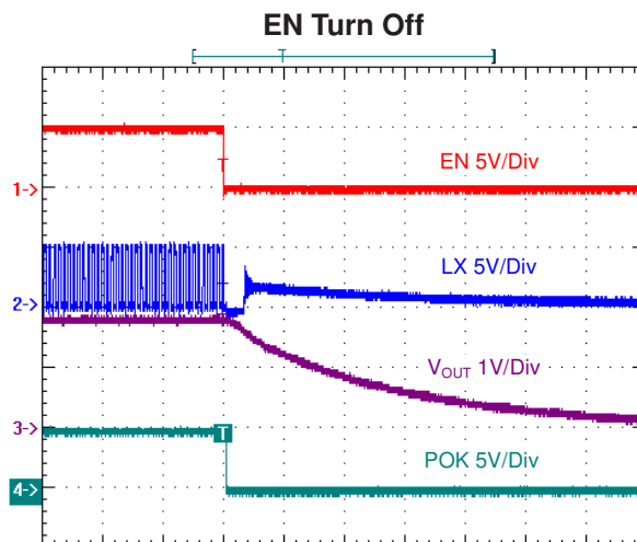
Time (10us/Div) V_{IN} = 5.0V , V_{OUT} = 1.8V , I_{OUT} = 3A
