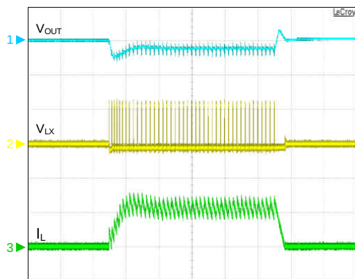
Load Transient 1
