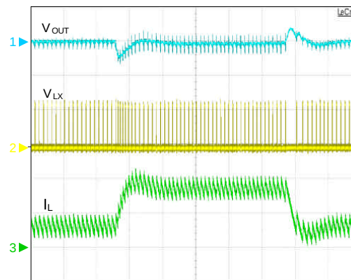
Load Transient 2
