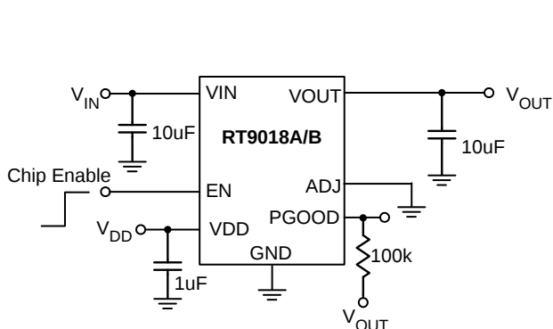
Figure 1. Fixed Voltage Regulator
