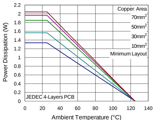
Figure 4. De-rating Curves
