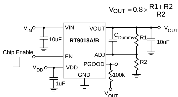
Figure 2. Adjustable Voltage Regulator
